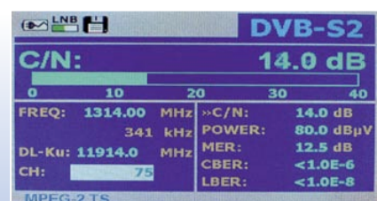
Carrier to Noise ratio measurement
